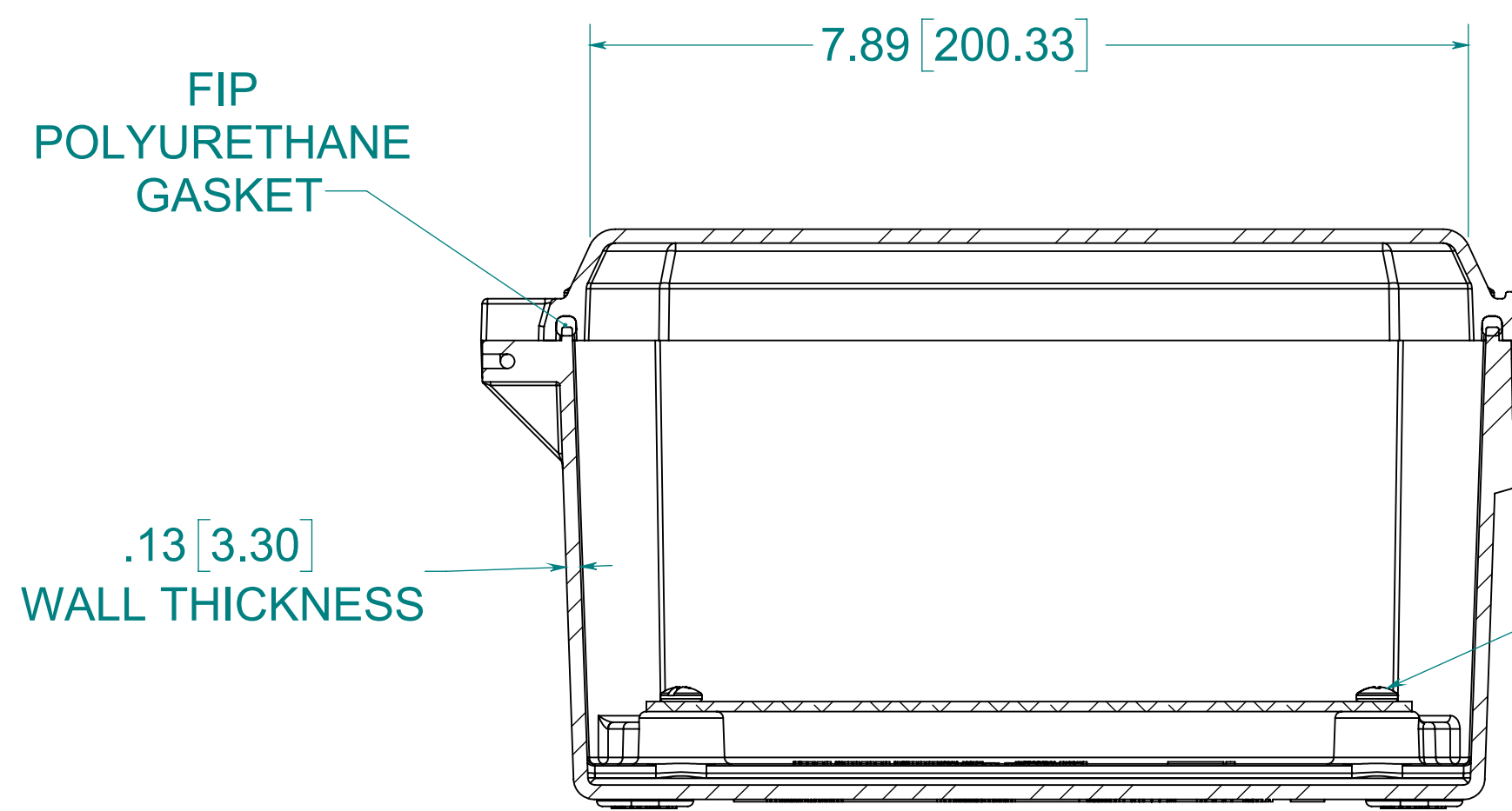
SECTION B-B
