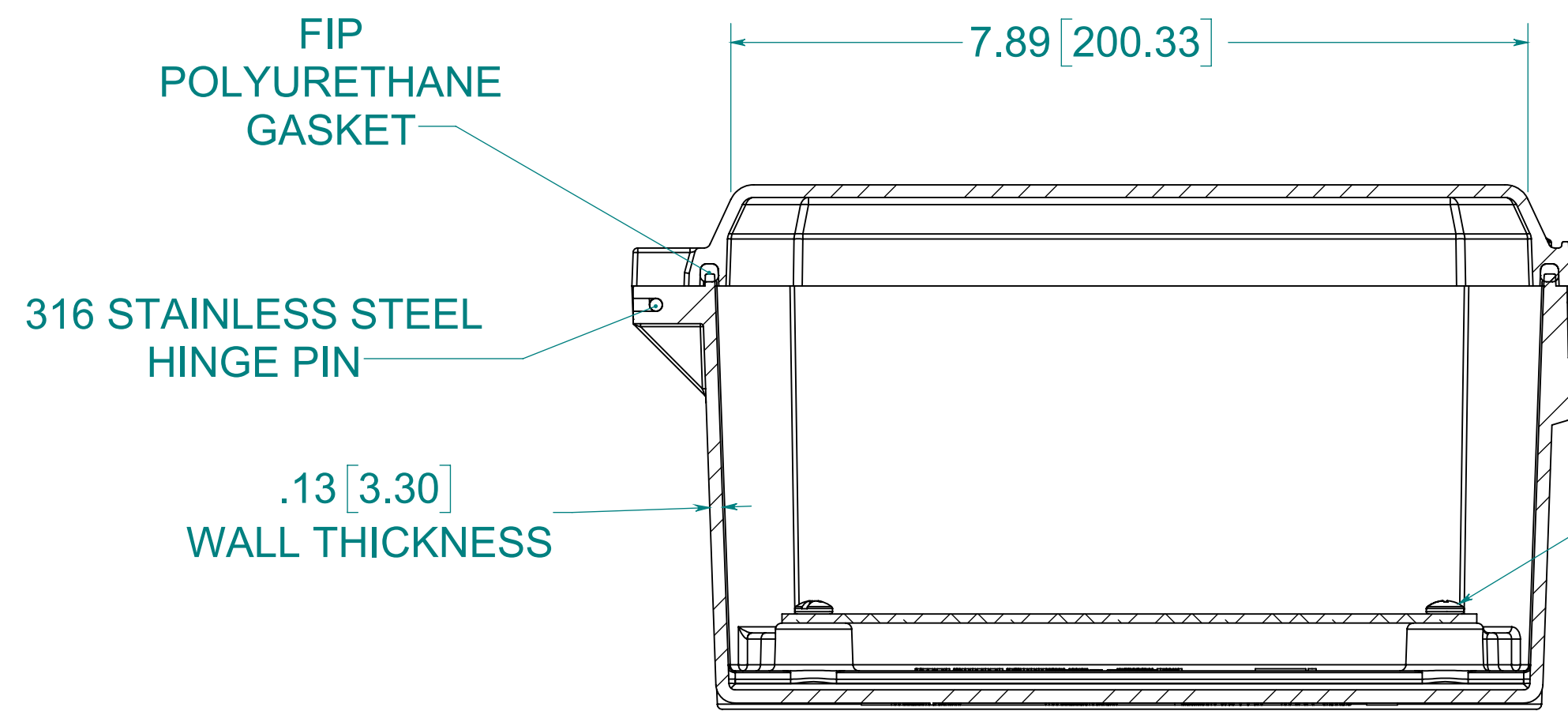
SECTION B-B
