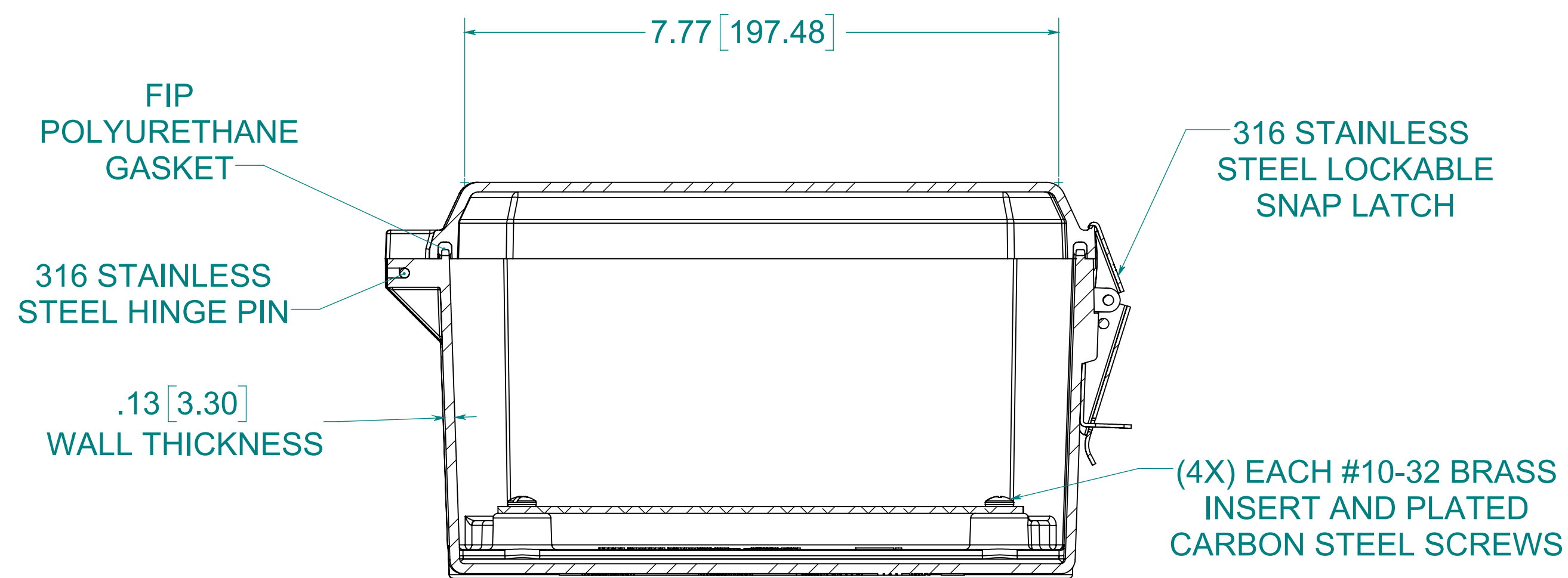
SECTION B-B
