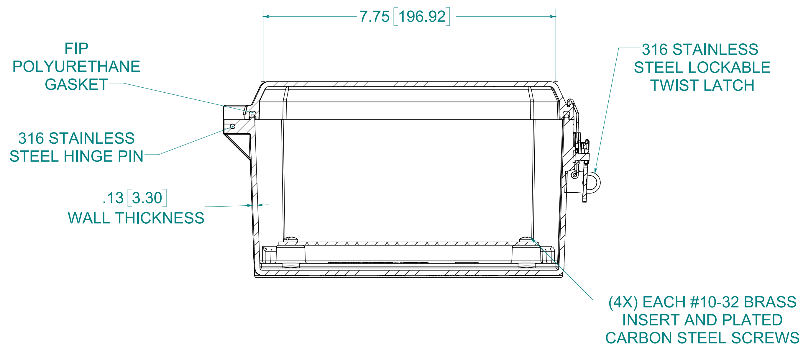
SECTION B-B
